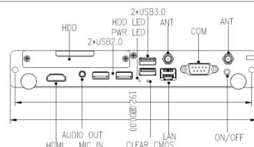
Rear Panel External I/O
